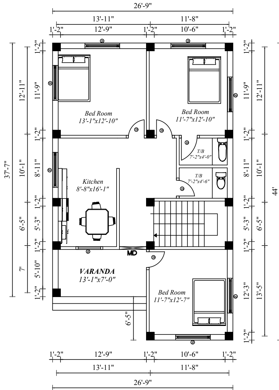
FIG :- GROUND FLOOR PLAN
