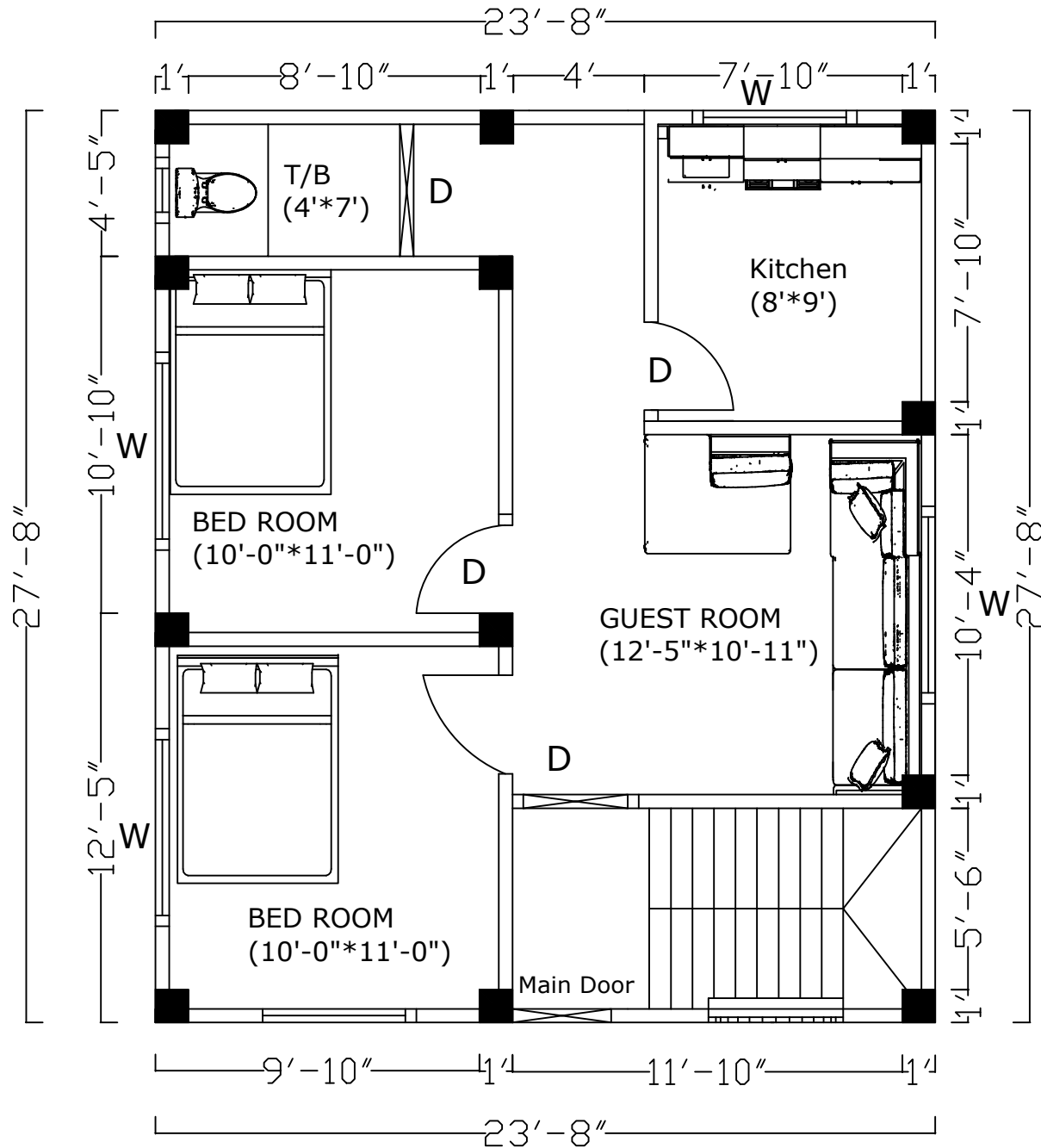
FLOOR PLAN
